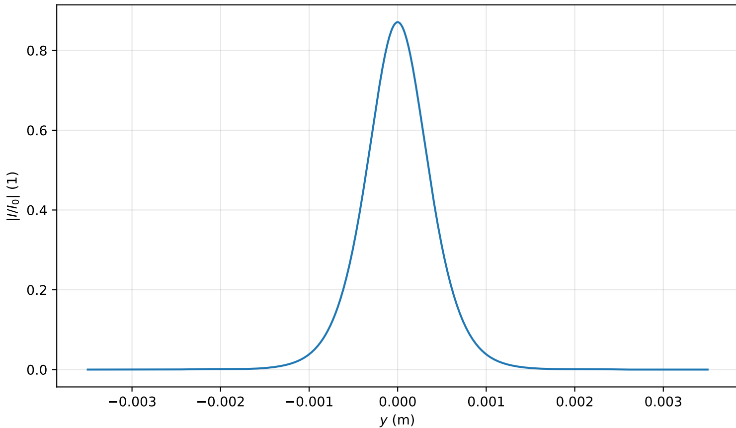
Intensity profile I(x=0, y, z=3.981)/I_0 , P_{in}=0.8P_{cr} , artificial time
